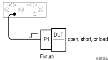
TDR DUT Reflection Measure
